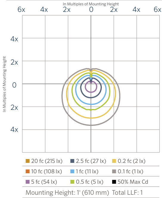
TD 1LED Isofootcandle Plot
