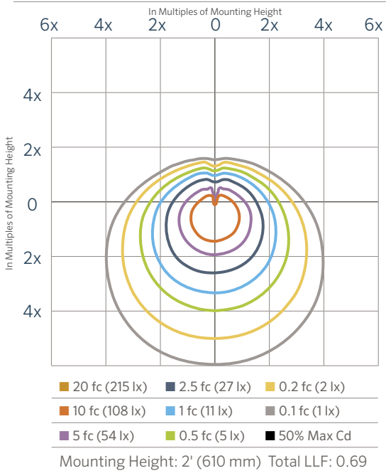
TD 6LED Isofootcandle Plot
