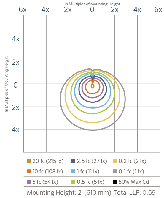
TD 3LED Isofootcandle Plot
